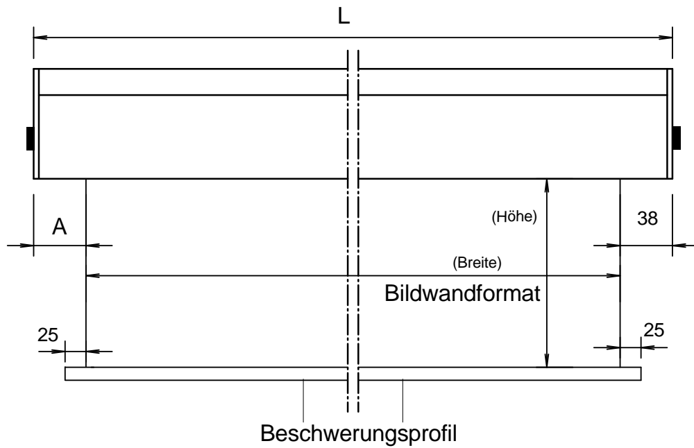
Wandmontage
